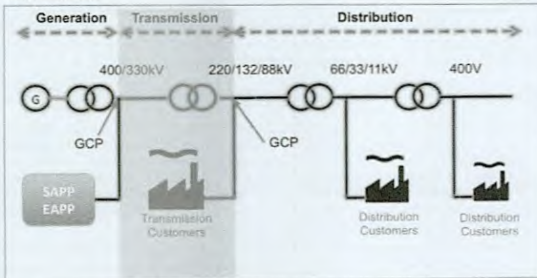
Figure 2.4.4.1: National Transmission Infrastructure
