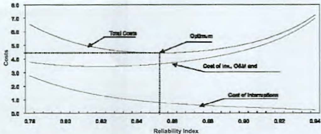
Figure 4.4.2: System Costs as a Function of System Reliability
